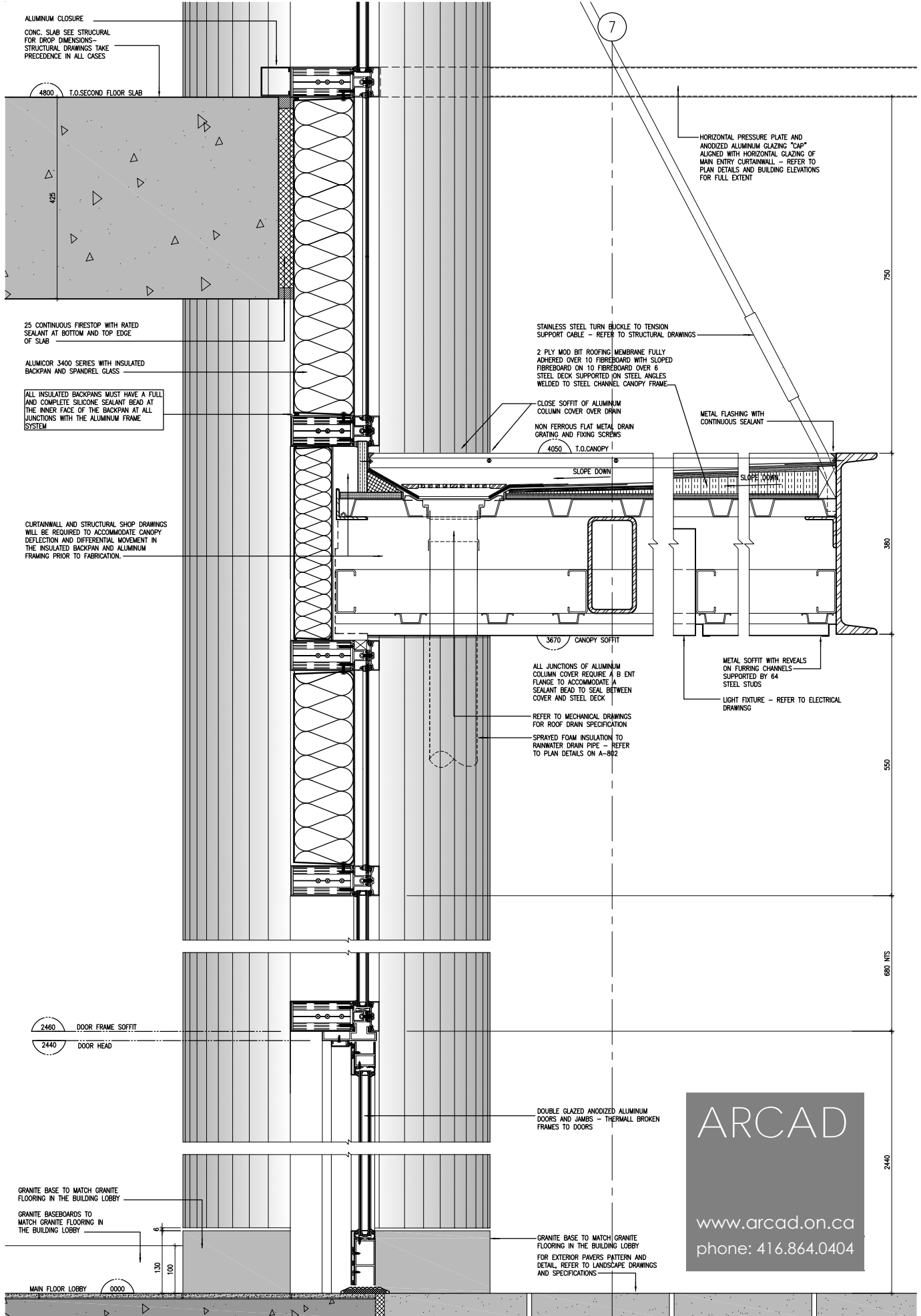
1 SECTION AT MAIN ENTRANCE DOORS AND CANOPY ABOVE A-803 SCALE: 1:5
